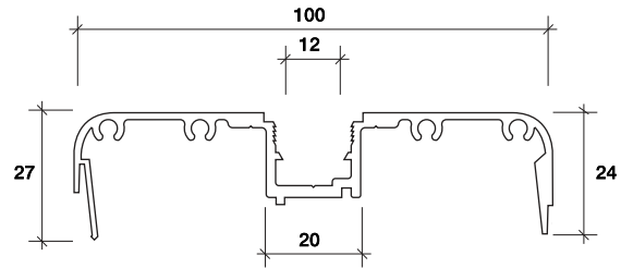
BACK-TO-BACK MULLION
