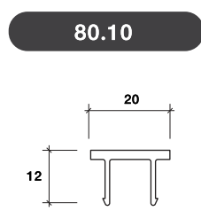
FLUSH STOP
