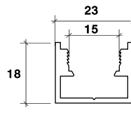
GLAZING CHANNEL
