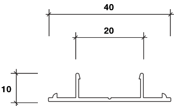
MULLION INFILL
