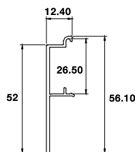
COVER PLATE
