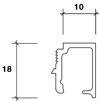
GLAZING BEAD
