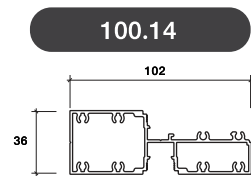
HORIZ MIDRAIL
