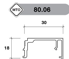
GLAZING BEAD
