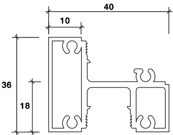
HORIZONTAL MULLION
