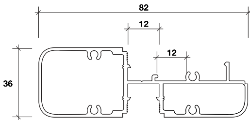
HORIZONTAL MULLION
