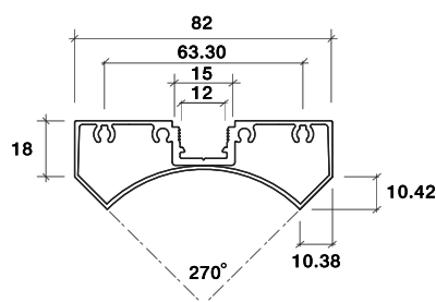
CURVE MULLION
