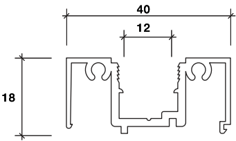
BACK-TO-BACK MULLION
