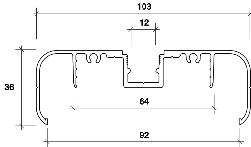
MULLION
