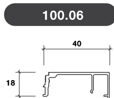
GLAZING BEAD
