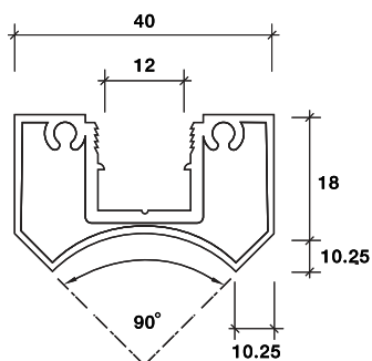
CURVE MULLION
