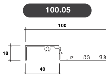
GLAZING MULLION
