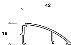
GLAZING BEAD
