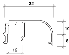
GLAZING BEAD
