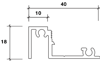
GLAZING MULLION
