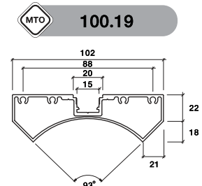
CURVE MULLION
