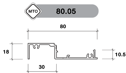
GLAZING MULLION
