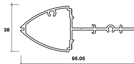
HORIZONTAL MULLION
