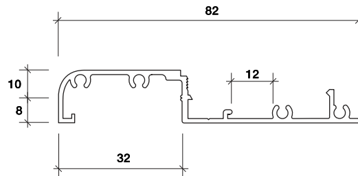
GLAZING MULLION
