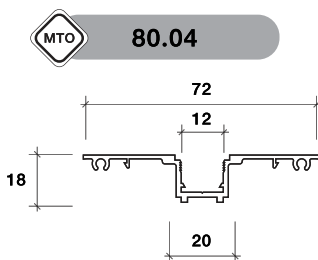
FRAME HEAD
