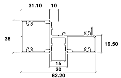
HORIZ MIDRAIL
