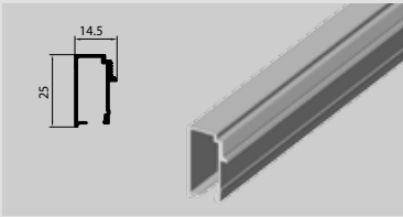
► LT.45-06 45 mm. Glazing Bead
