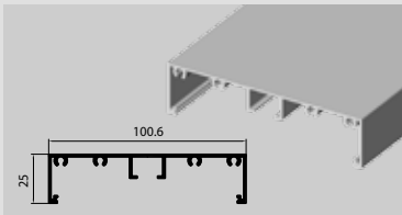
► LT.01 100 mm. Flat Mullion
