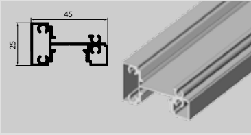
► LT.45-08 45 mm. Horizontal Midrail
