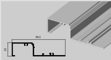
► LT.05 100 mm. Glazing Mullion
