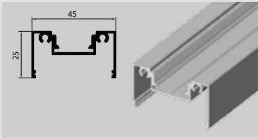
► LT.45-07 45 mm. Back to Back Mullion
