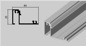
► LT.45-05 45 mm. Glazing Mullion
