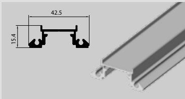
► LT.45-03 45 mm. Snap Back to Back Mullion
