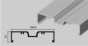
► LT.14 100 mm. Back to Back Mullion
