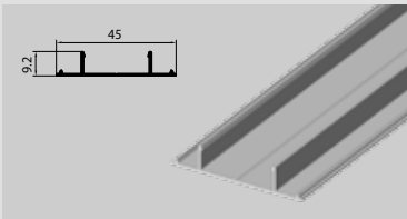
► LT.45-04 45 mm. Mullion Infill
