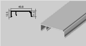
► LT.16 Glazing Bead Midrail
