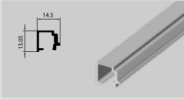
► LT.45-09 45 mm. Glazing bead Midrail
