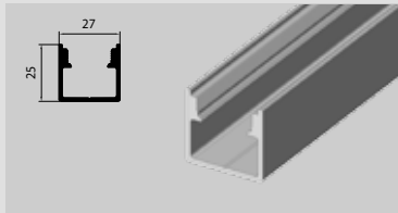
► LT.17 25 mm. U channel
